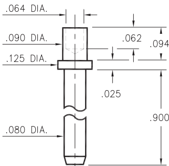
3233-2-00-XX-00-00-08-0 Swage mount in .094 hole. For .062 thick board.
