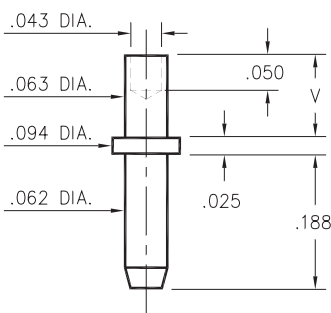
3144-X-00-XX-00-00-08-0 Swage mount in .067 hole.
